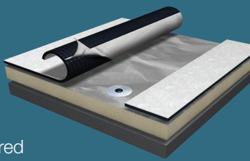
TPO Fully Adhered with Solvent-Based Adhesive
