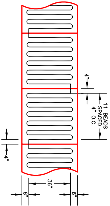
FIGURE 1 INSTALLATION USING 4" O.C. BEADS ON 4' X 4' BOARDS
