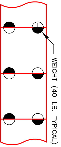
FIGURE 1 INSTALLATION USING 4" O.C. BEADS ON 4' X 4' BOARDS
