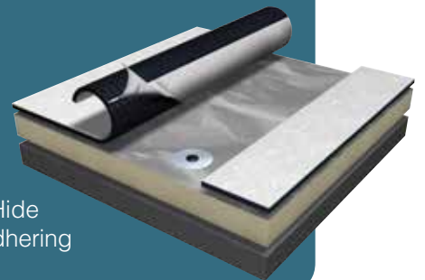
Mule-Hide Mechanically Attached
