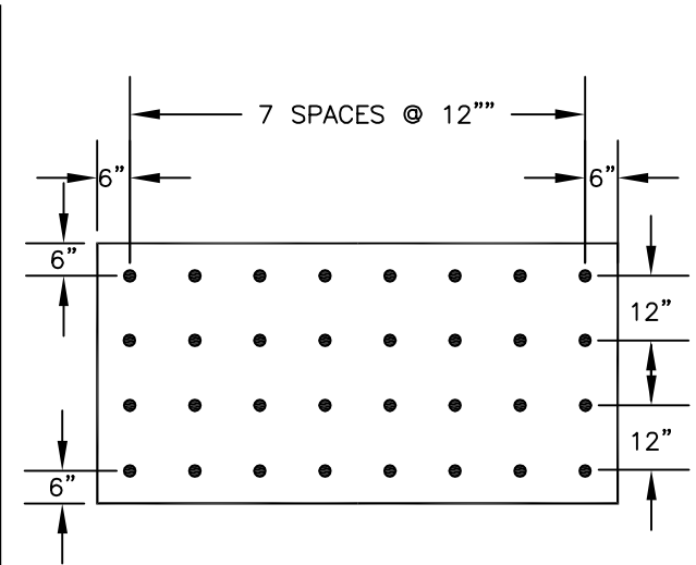
CORNERS (32) 1 FASTENER PER EVERY 1 SQ. FT.
