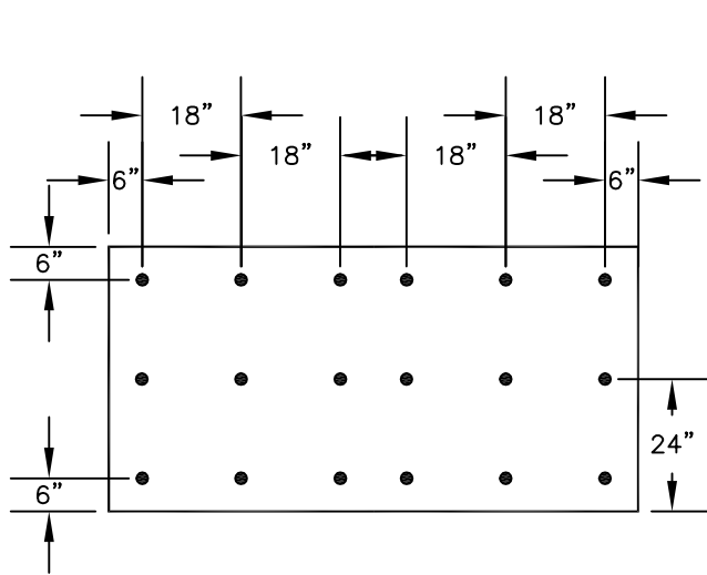
PERIMETER (18) 1 FASTENER PER EVERY 1.77 SQ. FT.
