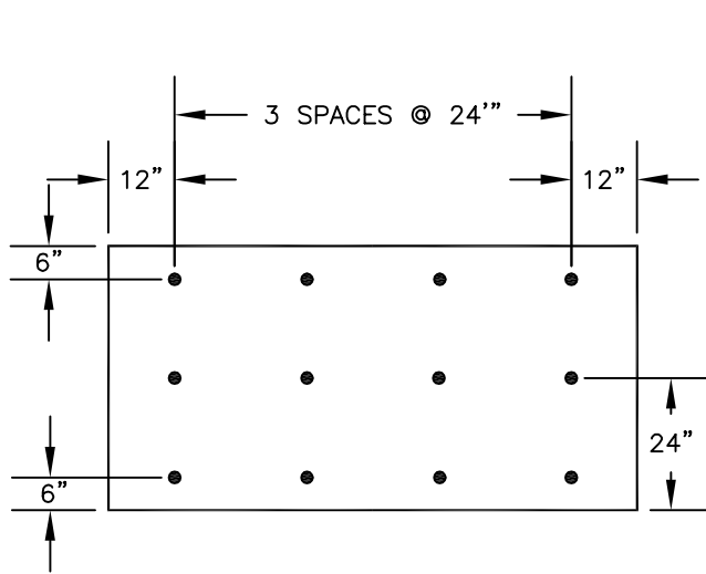
FIELD (12) 1 FASTENER PER EVERY 2.66 SQ. FT.
