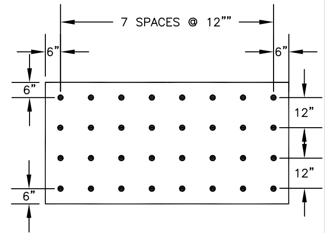
CORNERS (32) 1 FASTENER PER EVERY 1 SQ. FT.
