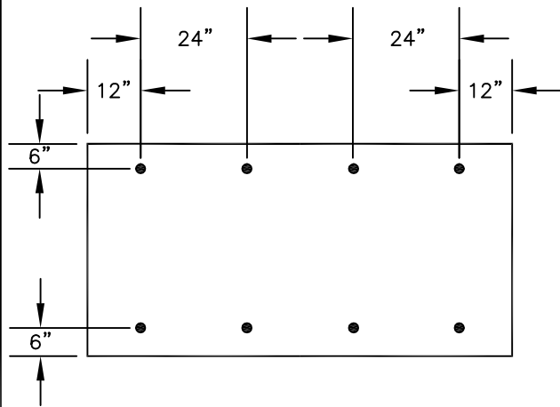
FIELD (8) 1 FASTENER PER EVERY 4 SQ. FT.
