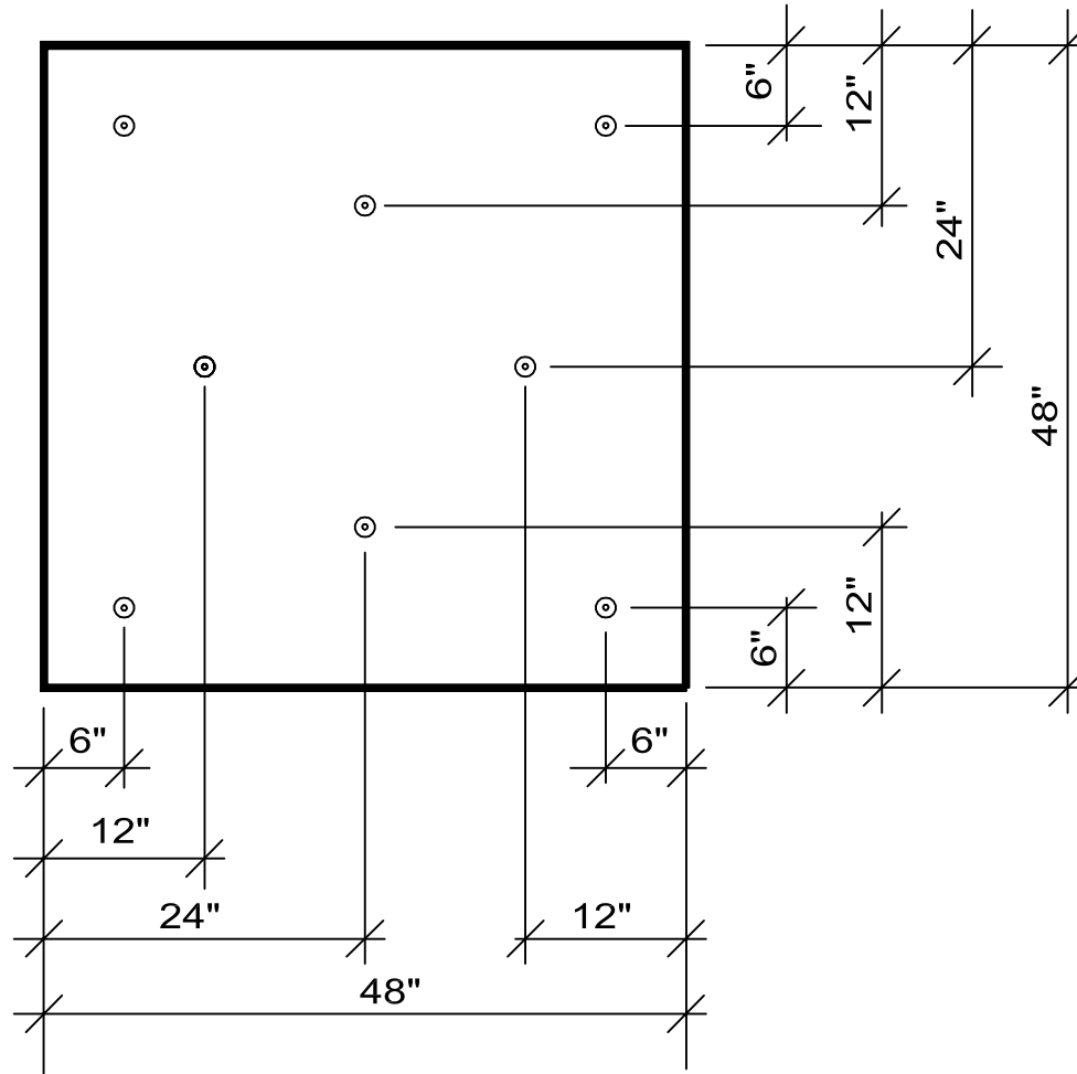
4' X 4' INSULATION ATTACHMENT (1 PER 2 SF.) STANDARD ATTACHMENT
