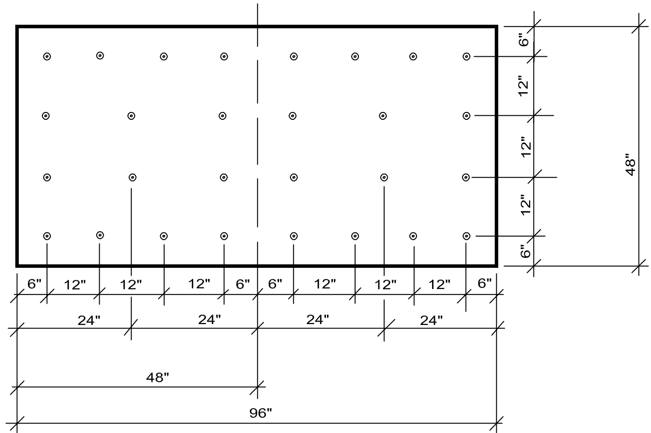
4' X 8' INSULATION ATTACHMENT (1 PER 1.14 SF) STANDARD ATTACHMENT (28 PER BOARD)
