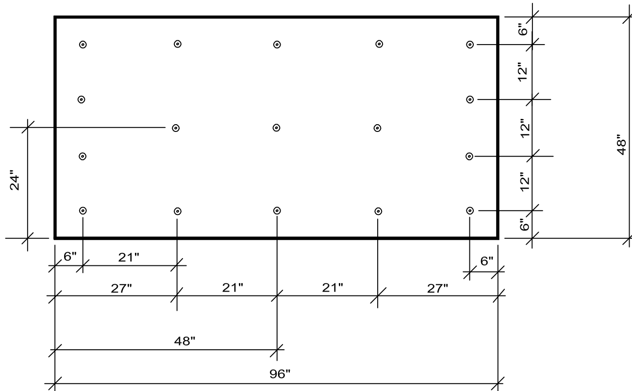
4' X 8' ORIENTED STRAND BOARD ATTACHMENT (1 PER 1.88 SF) STANDARD ATTACHMENT (MINIMUM 7/16" THICK)
